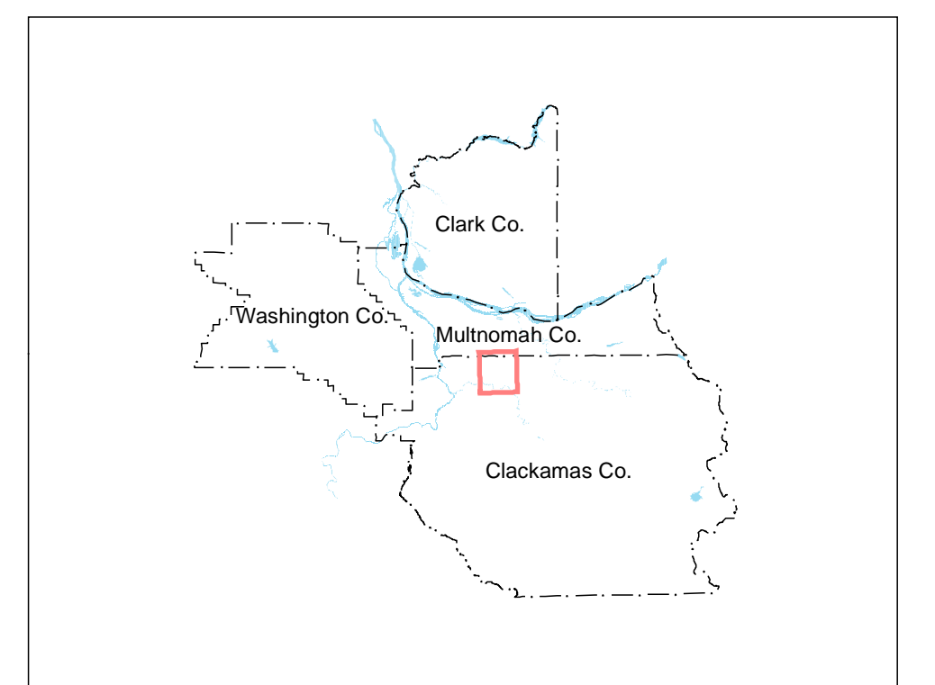
Location Map
